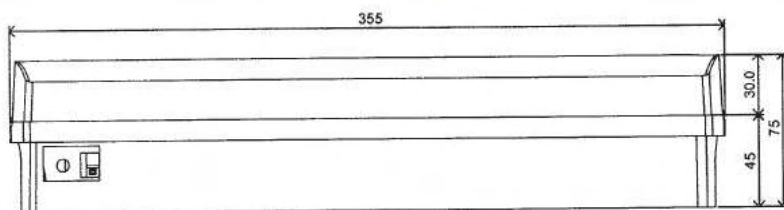
FRONT VIEW (in mm)
