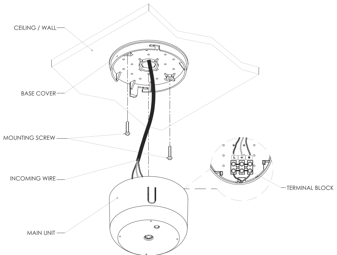
INSTALLATION OF PTH 100
